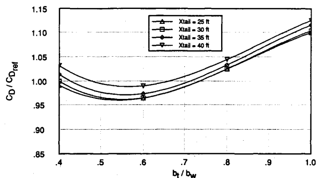
Fig. 13 Relative drag vs span ratio and tail length (symmetric box, fixed weight).
