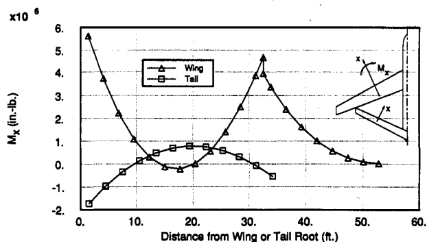
Fig. 7 Moment distribution M_x (typical joined wing).
