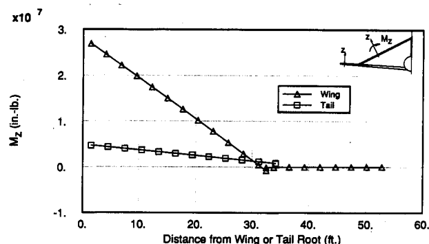
Fig. 8 Moment distribution M_z (typical joined wing).
